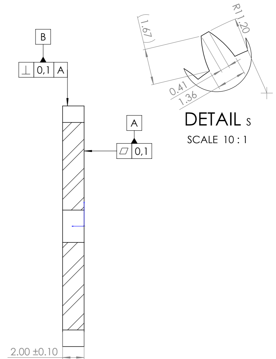
SECTION K-K
